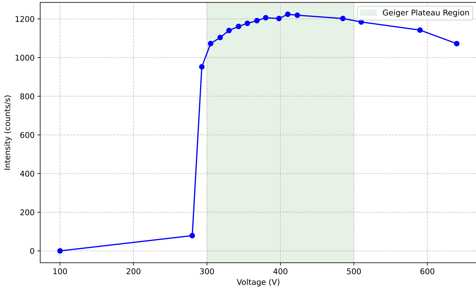
Geiger-Müller Counter Plateau Curve
