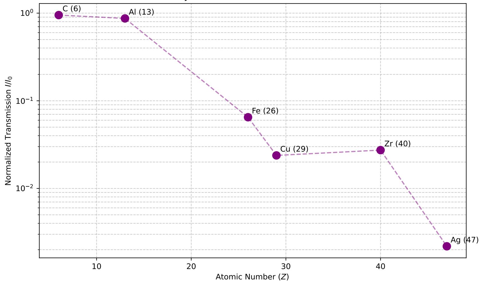
X-Ray Transmission vs. Atomic Number
