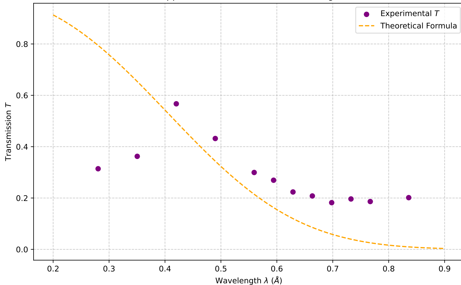
Copper Foil Transmission vs. Wavelength
