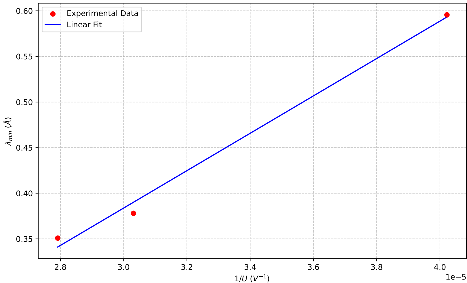
Duane-Hunt Law: \lambda_{min} vs 1/U
