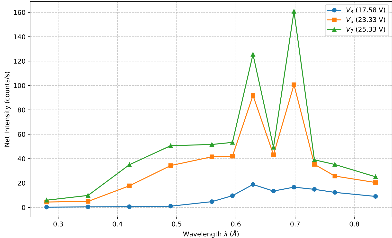
X-Ray Diffraction Spectra of LiF Crystal
