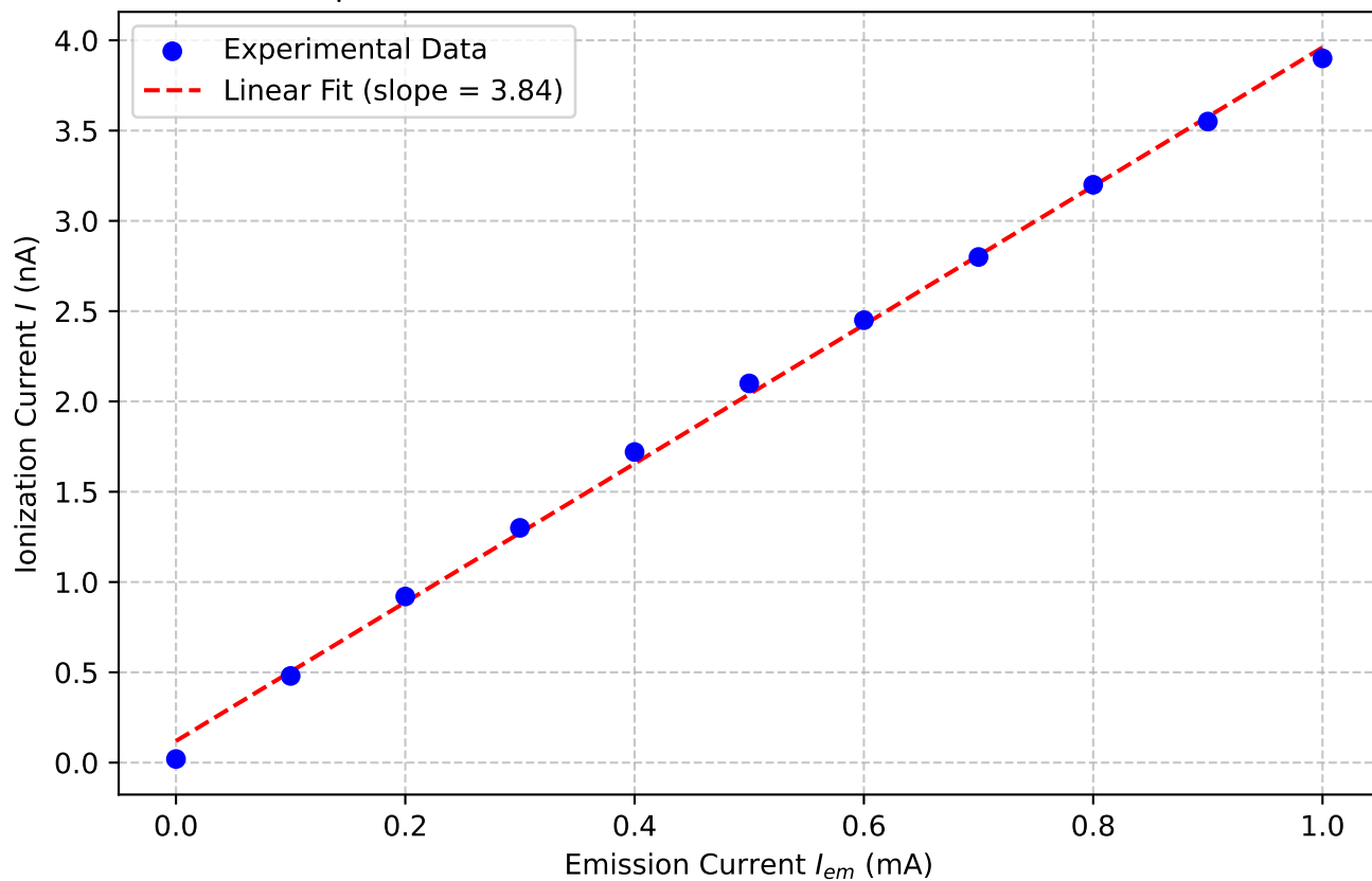
Experiment 2: Ionization Current vs. Emission Current
