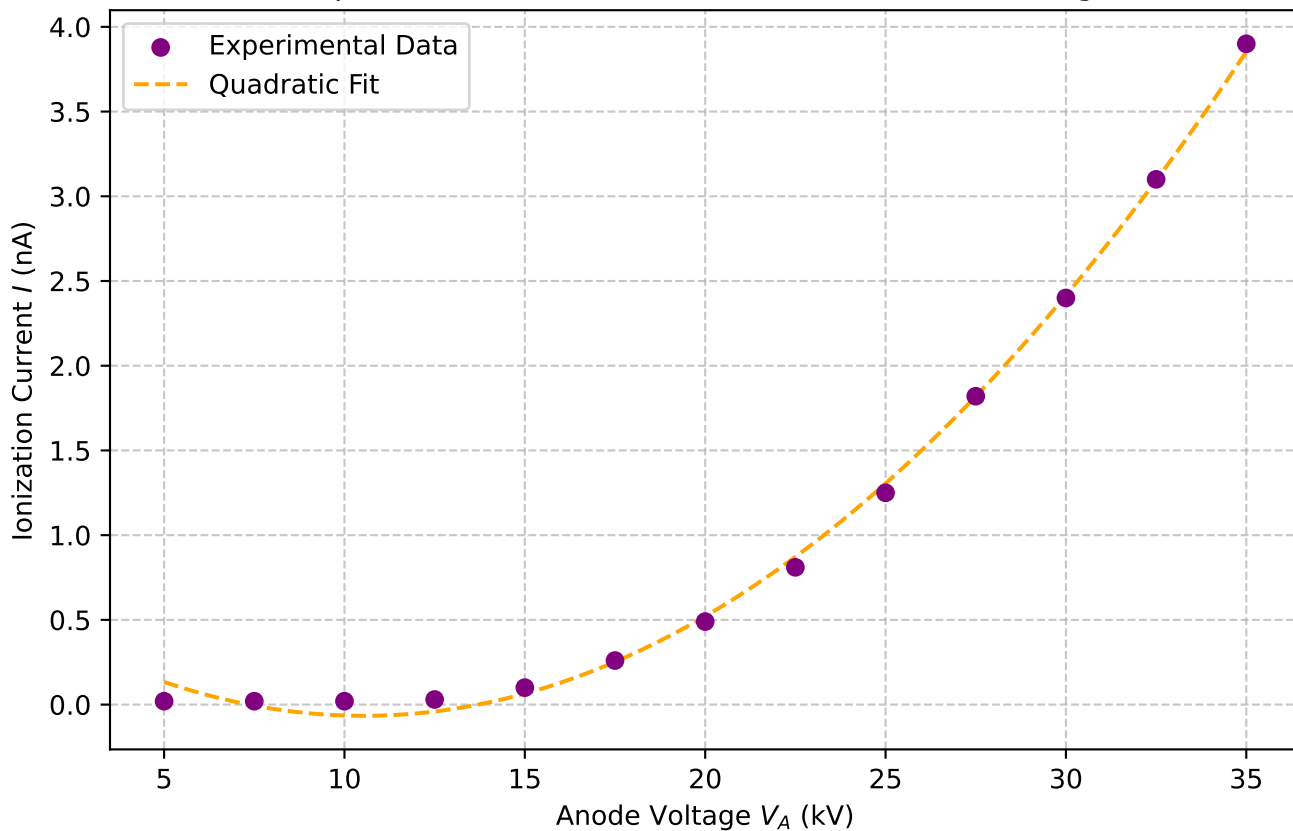
Experiment 3: Ionization Current vs. Anode Voltage
