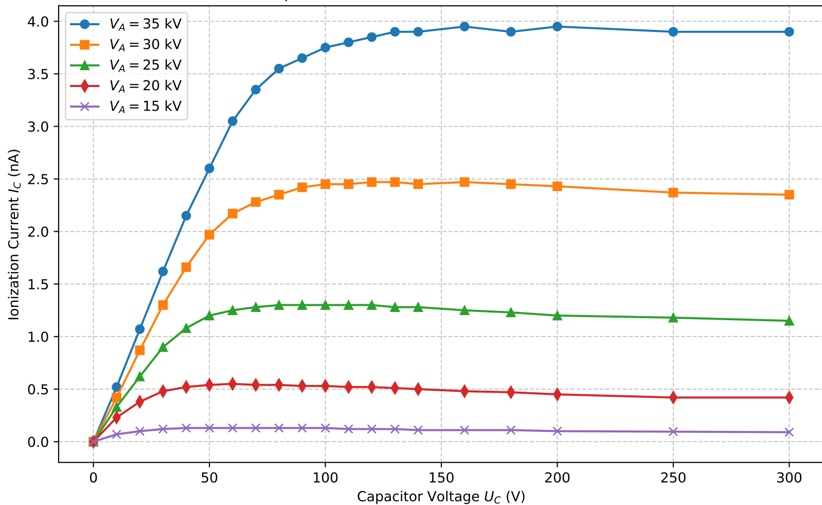
Experiment 1: Ionization Saturation Curves
