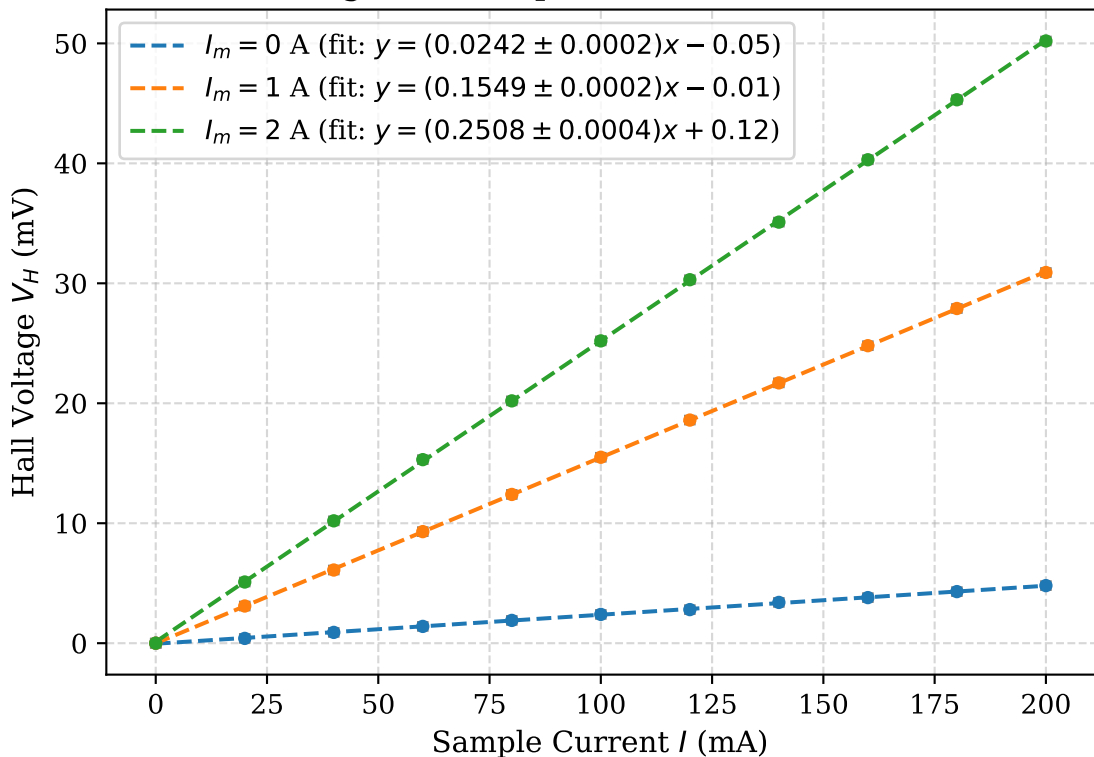
Hall Voltage vs. Sample Current with Error Bars
