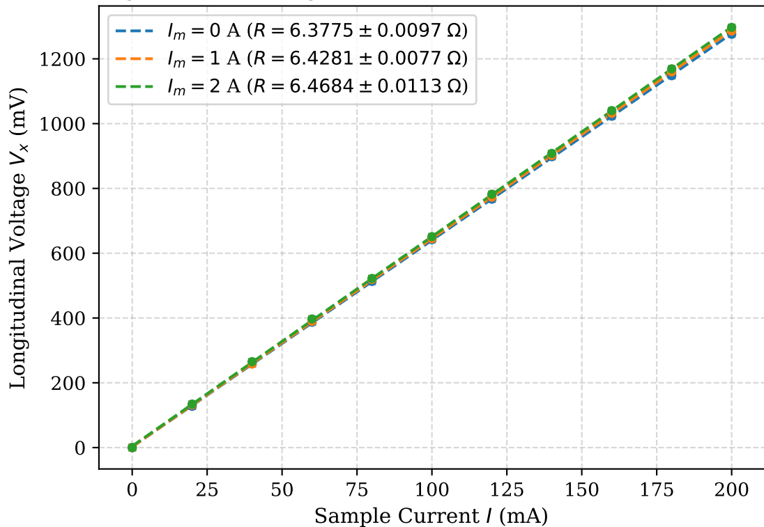
Longitudinal Voltage vs. Sample Current with Error Bars
