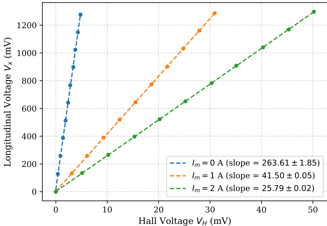
Longitudinal Voltage vs. Hall Voltage with Error Bars
