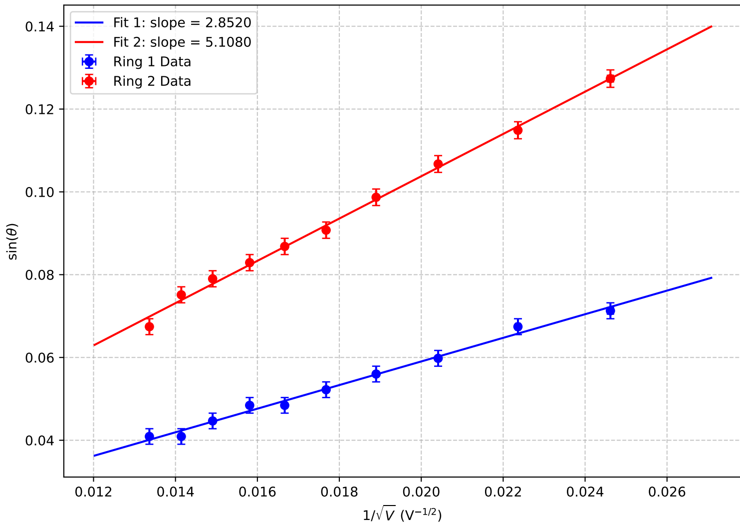
Bragg Diffraction: \sin(\theta) vs. 1/\sqrt{V}
