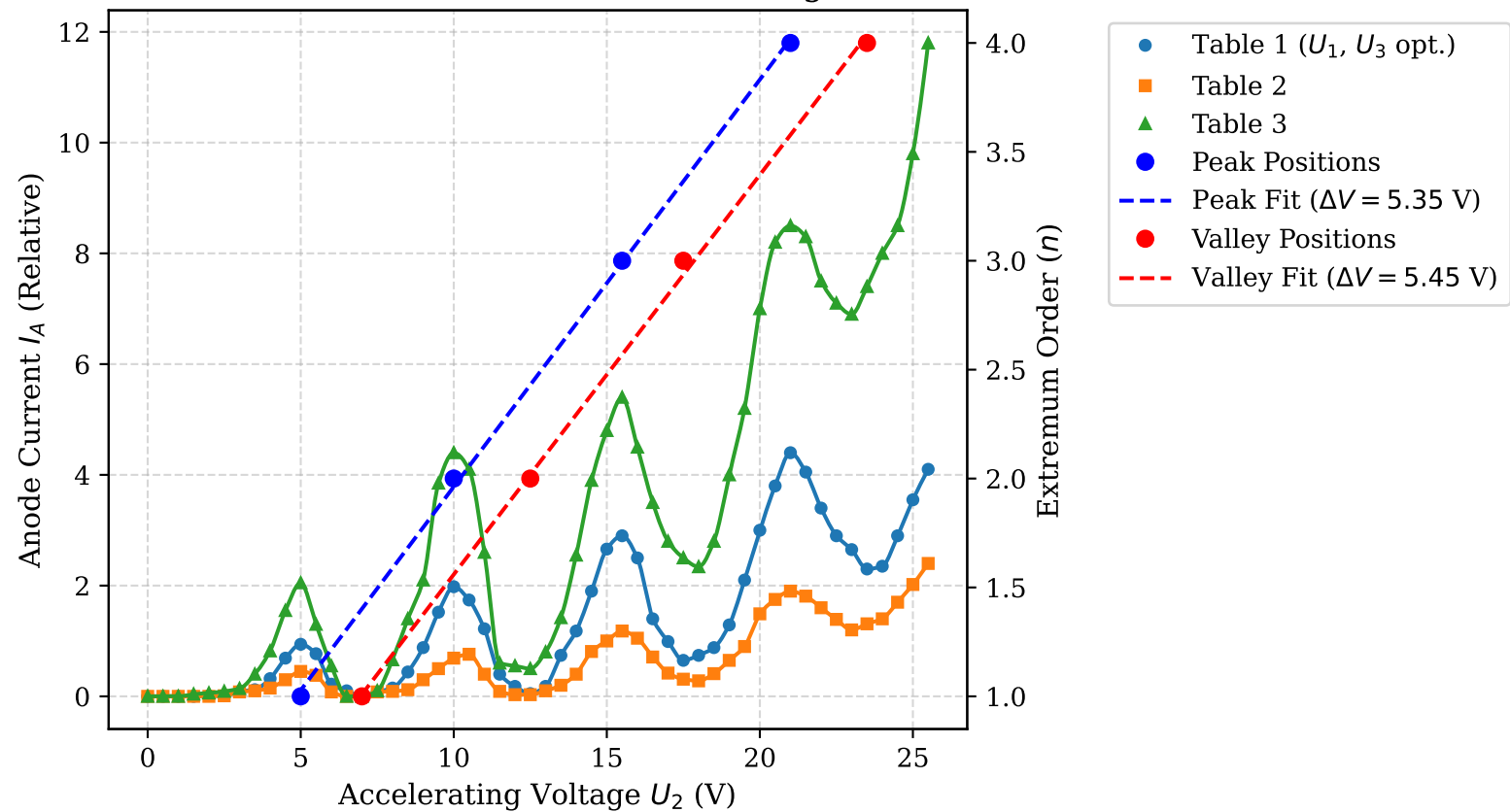
Franck-Hertz I-V Curves & Extrema Regression
