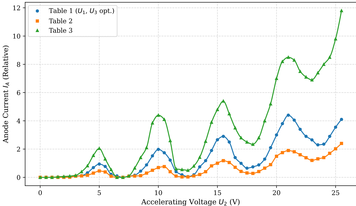
Franck-Hertz I-V Curves
