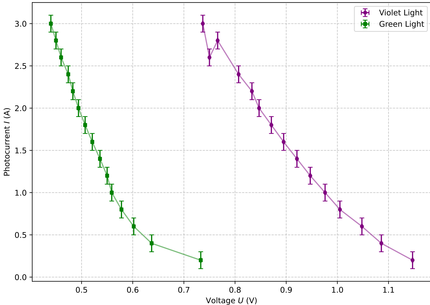
Photocurrent vs. Retarding Voltage
