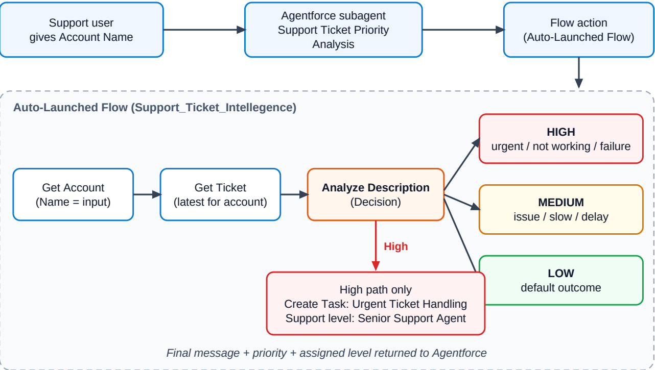
Figure 7.1 – Solution architecture and data flow
