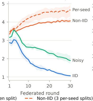
(b) Conditional GAN, Sync-G
