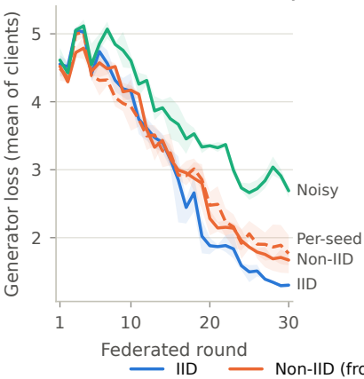
(a) Unconditional GAN, Sync-G
