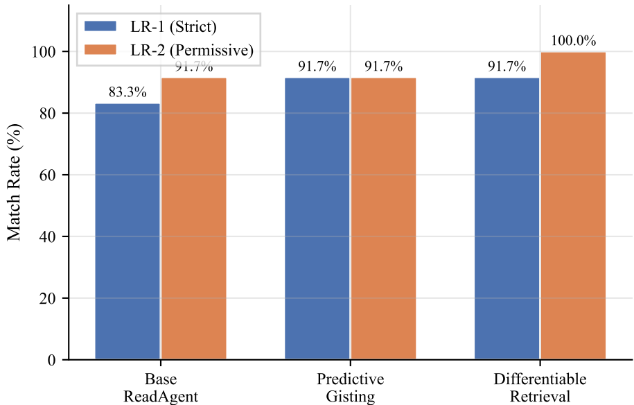
LLM Rating Comparison (Aggregated)
