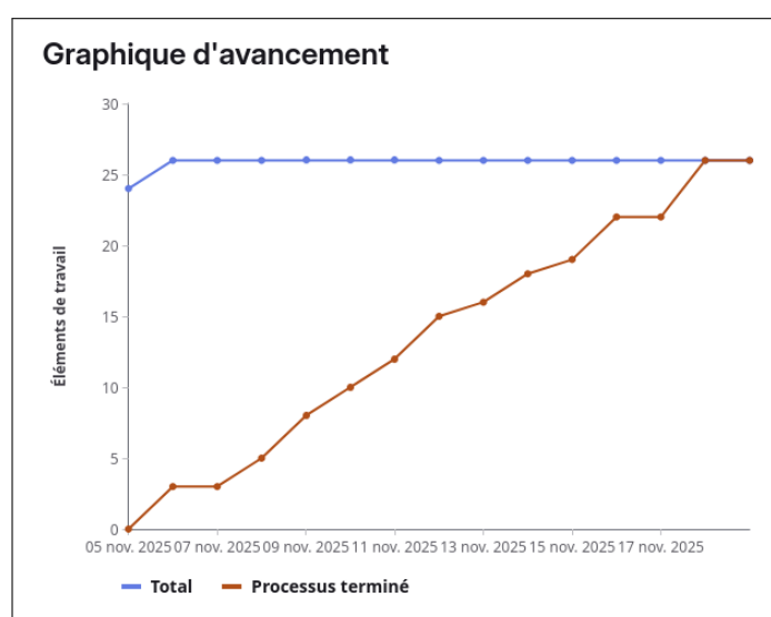
FIGURE 1.6 – Burn up chart
