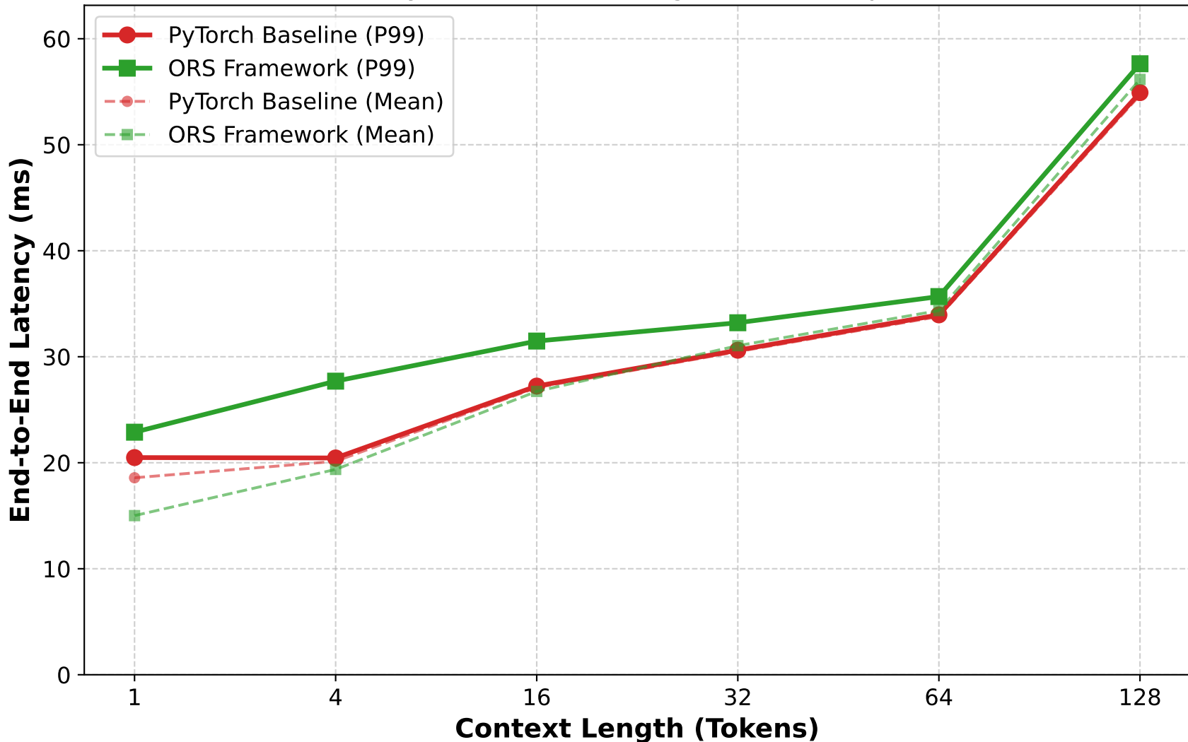
Latency vs. Context Length (1000 requests)
