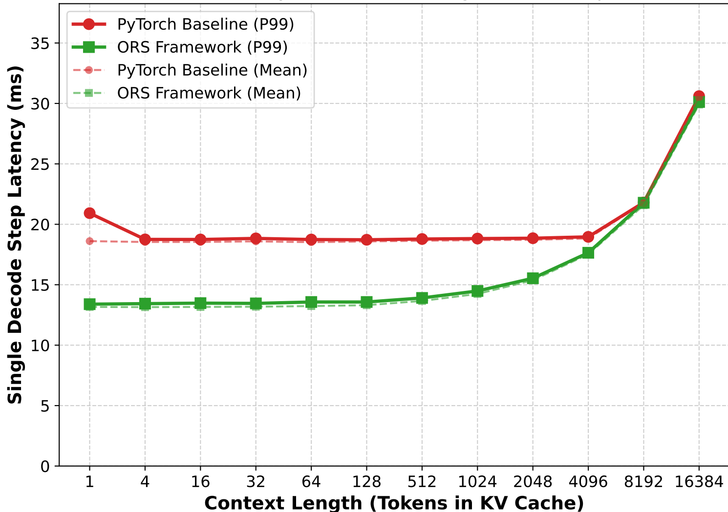
Decode Latency vs. Context Length (1000 requests)
