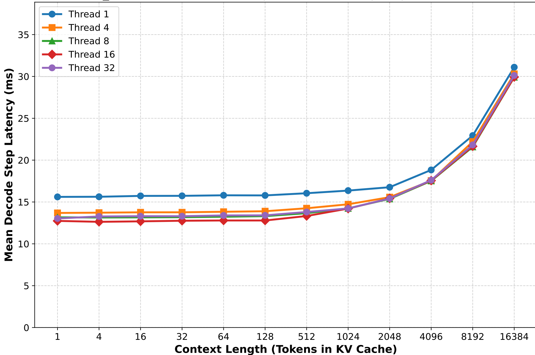
ORS_Framework: Mean Latency vs. Context Length by Thread Count
