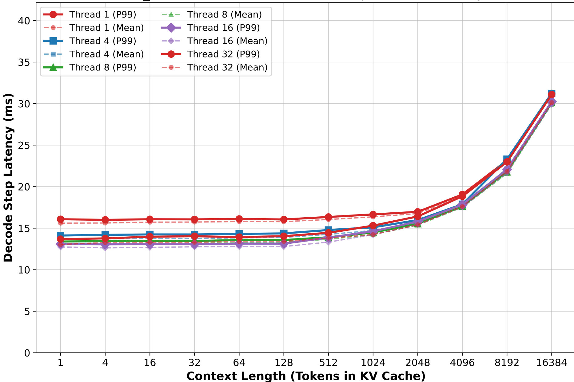
ORS_Framework: Multi-Thread Latency vs. Context Length
