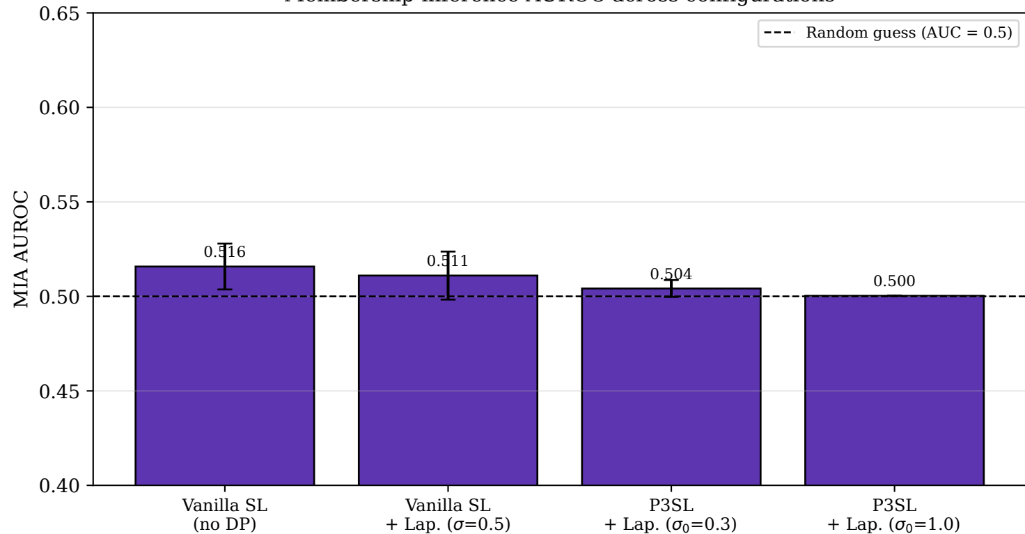
Membership-inference AUROC across configurations
