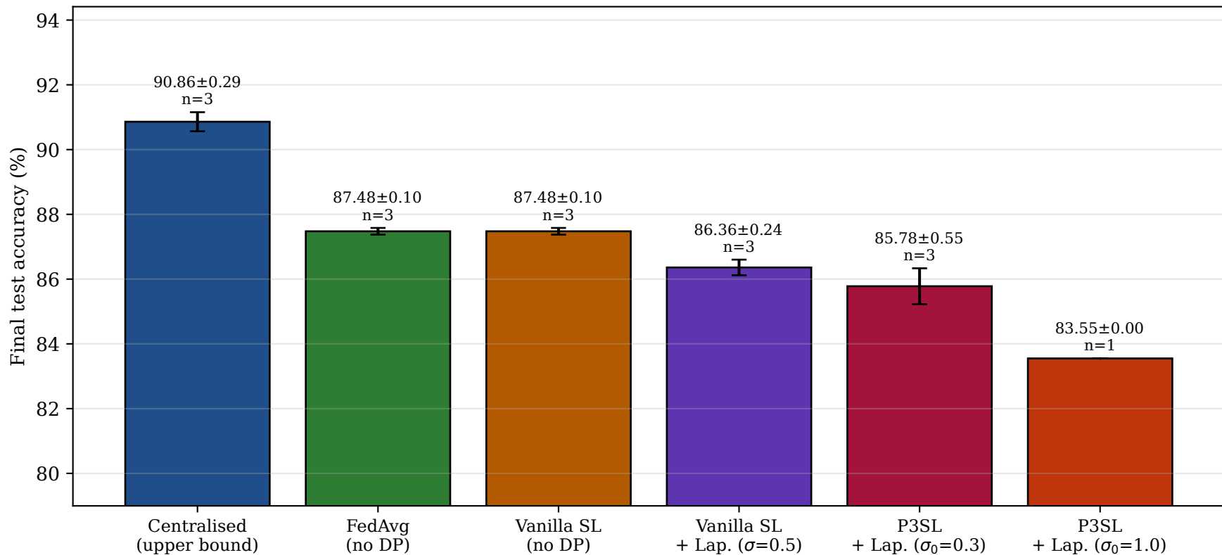
Final accuracy across configurations (FashionMNIST, 30K subset, 25 rounds)
