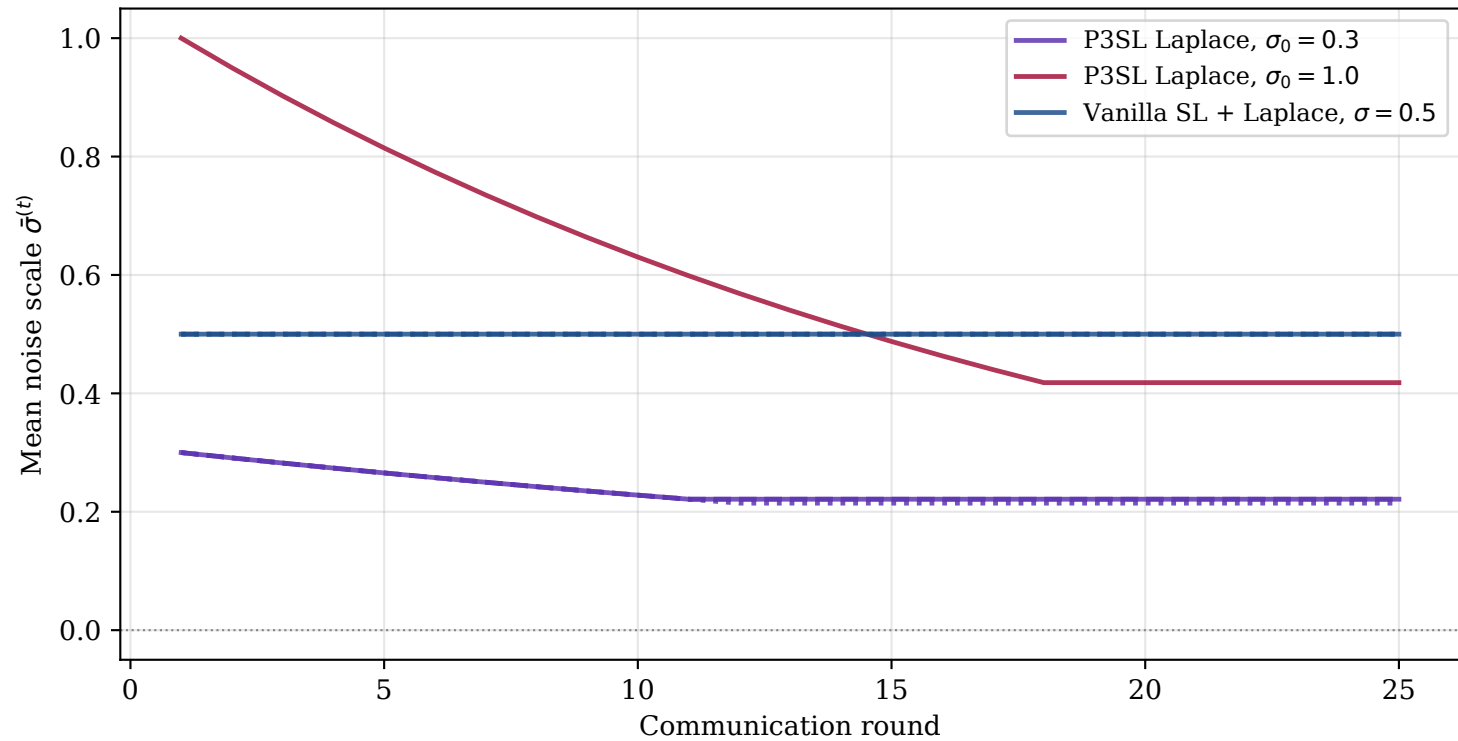
Noise scale trajectory under the bi-level loop (one line per seed)
