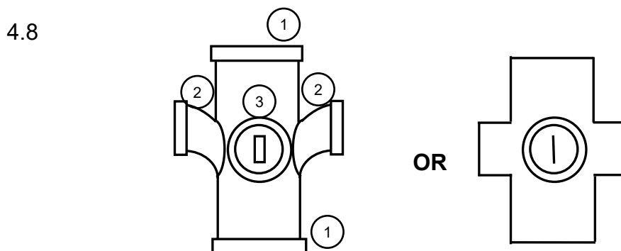
CROSS-JUNCTION 90° DOUBLE REDUCING WITH INSPECTION EYE
