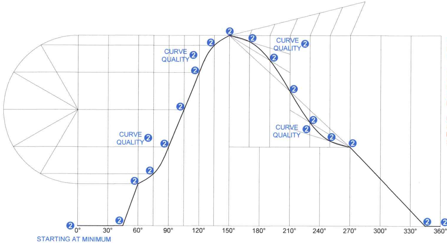
DISPLACEMENT GRAPH 3 SCALE 156 = 360° 3
