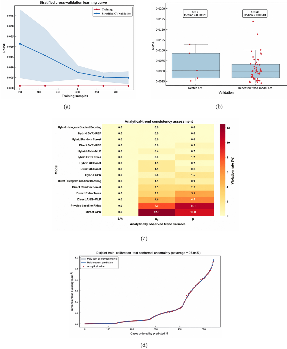
Figure 8. Uncertainty and validation of machine learning (ML): (a) stratified cross-validation (CV) learning curve; (b) root mean square error (RMSE) stability across validation folds; (c) analytical-trend consistency assessment; (d) disjoint train-calibration-test conformal uncertainty (coverage = 97.04%)
