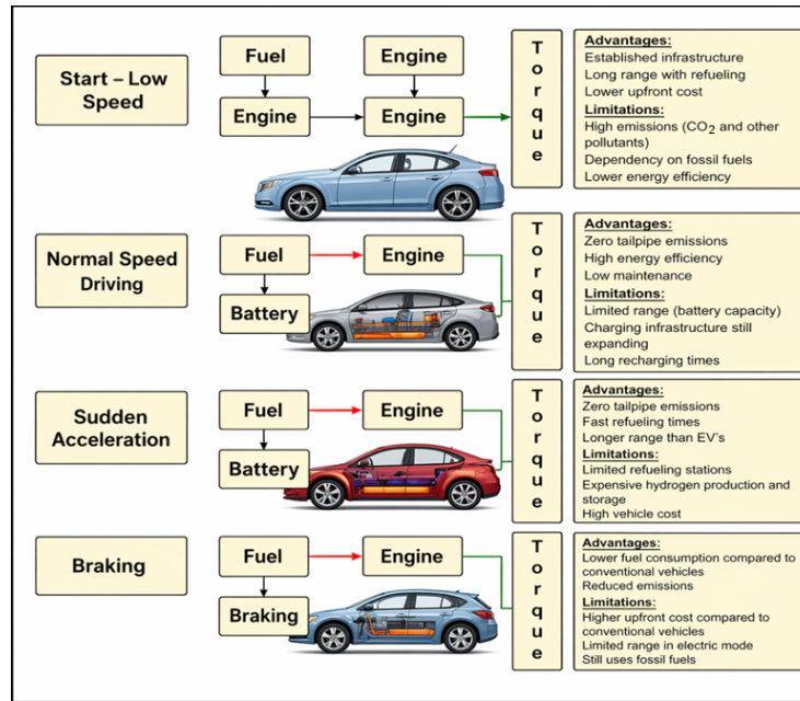
Figure 3. Power flow and torque contribution of hybrid electric vehicles (HEVs) during start, normal driving, acceleration, and braking Note: EV (electric vehicle).
