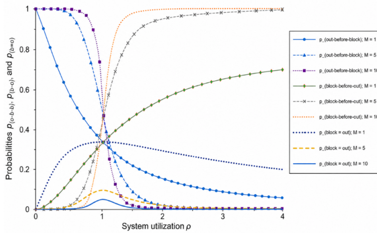
Figure 3. Probabilities p_{(\text{out-before-block})} , p_{(\text{block-before-out})} , and p_{(\text{block} = \text{out})} vs. utilization \rho for a supply-demand warehouse
