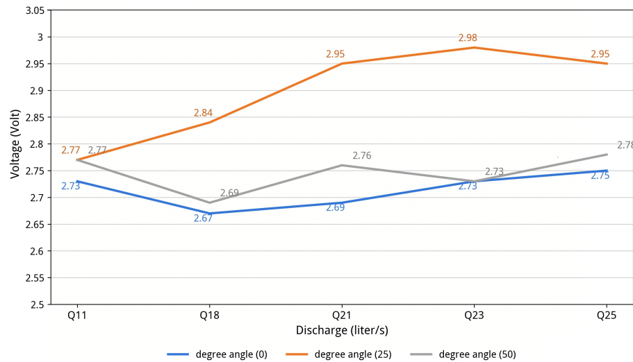
Figure 7. Angles of 0^\circ, 25^\circ, 50^\circ with discharge variations of 11, 18, 21, 23, and 25 L/s against voltage
