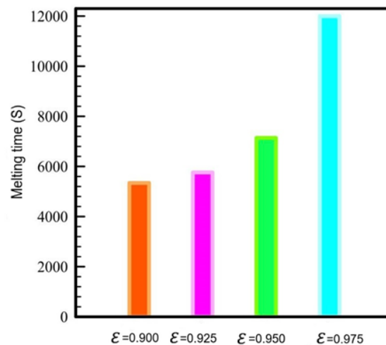
Figure 4. The melting time when the melting volume fraction (MVF) reaches 0.95 for different porosity values, adapted from Ref. [40]
