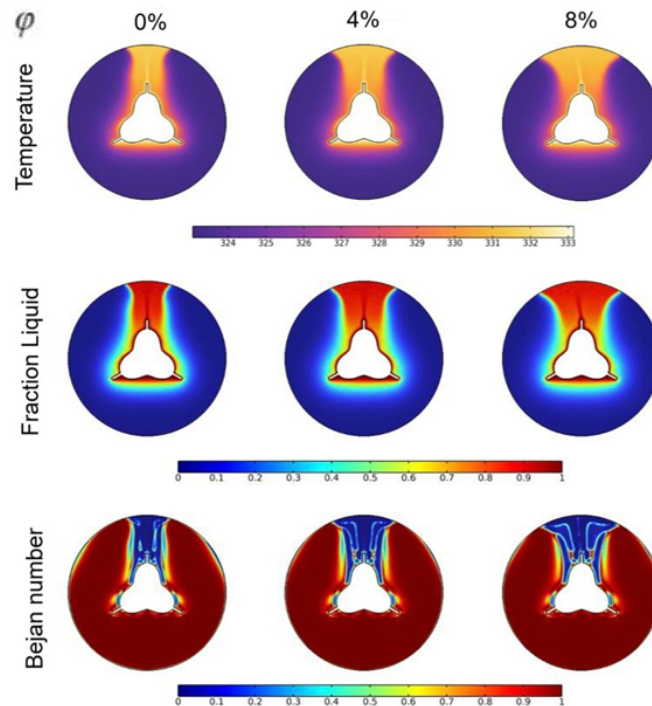
Figure 11. Temperature contours, liquid fraction, and Bejan number for different nanoparticle concentrations (0%, 4%, and 8%) after 20 minutes of thermal exposure, adapted from Ref. [76]
