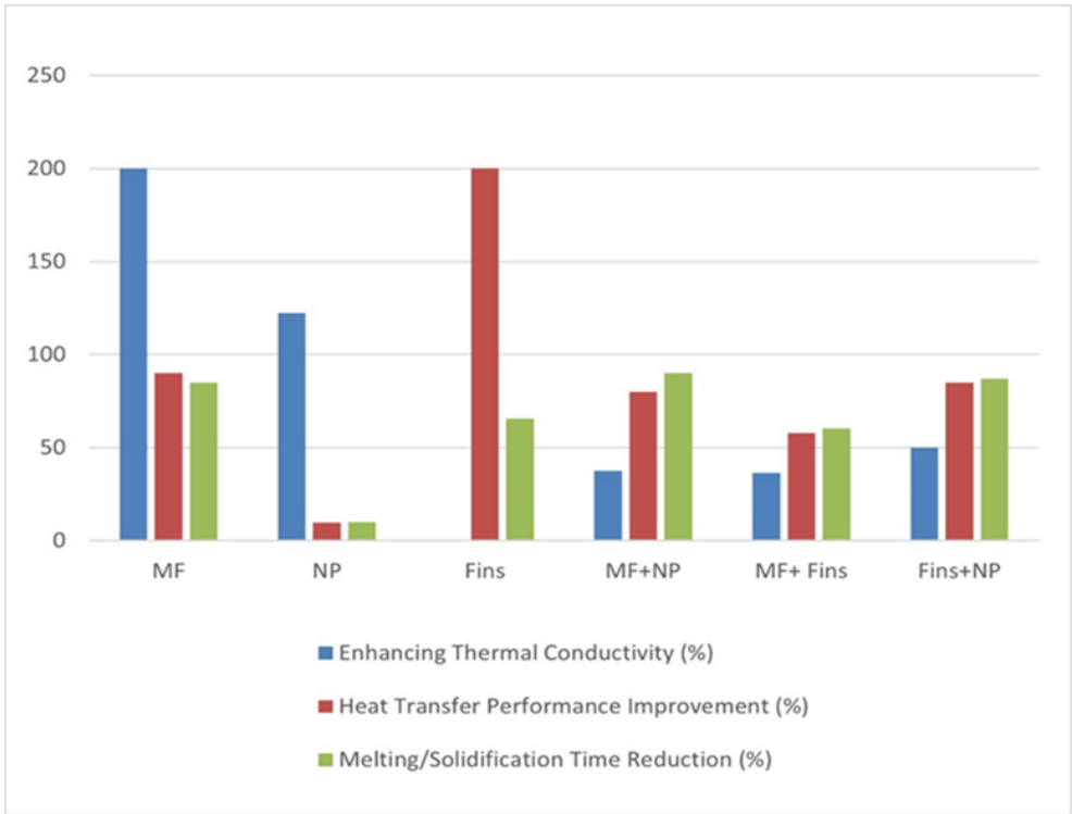
Figure 12. Comparison of phase change material enhancement techniques Note: MF = metal foam; NP = nanoparticle.
