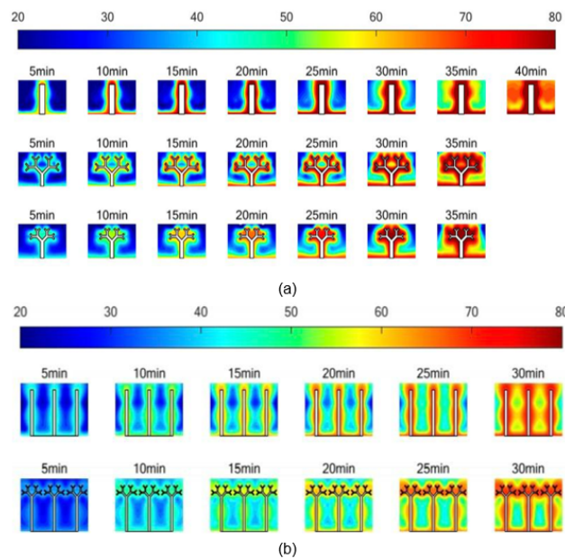
Figure 7. Temperature distribution of units (a) with one fin; (b) with three fins, adapted from Ref. [63]
