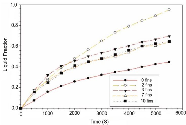
Figure 8. Liquid fraction phenomena of different fin arrangements (0, 2, 3, 7, and 10 fins) as a function of time, adapted from Ref. [66]
