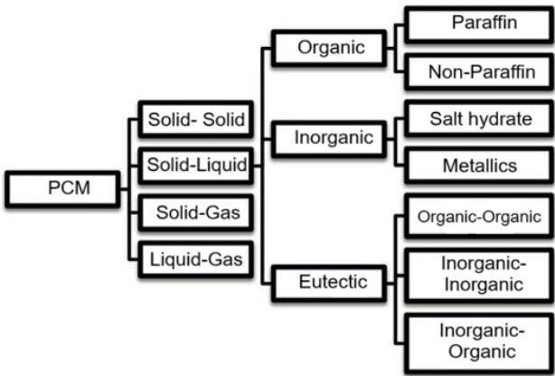
Figure 1. Classification of phase change material (PCM) based on their thermal storage capacities, phase transition temperature, thermal properties, and material type, adapted from Ref. [15]
