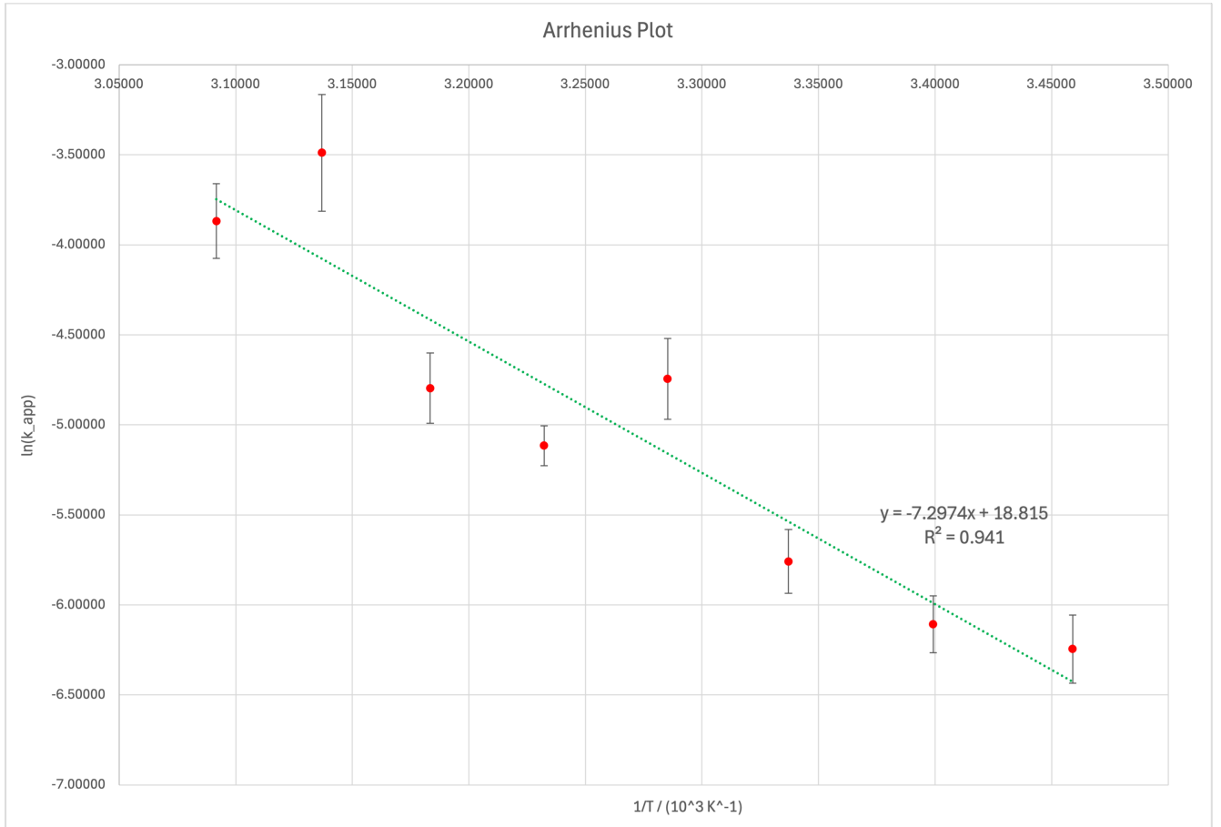
Figure 4: Arrhenius plot, graph of \ln k_{app} vs. \frac{1}{T} \cdot 10^3 .
