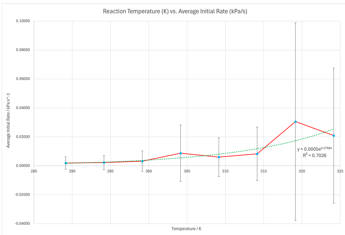
Figure 3: Graph of average initial rate ( \text{kPa s}^{-1} ) vs. temperature level (K).
