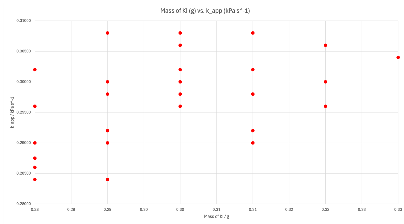
Figure 5: Graph of mass of KI vs. k_{app} for all trials.
