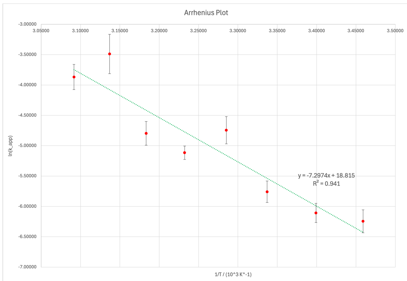
Figure 4: Arrhenius plot, graph of \ln k_{app} vs. \frac{1}{T} \cdot 10^3 .
