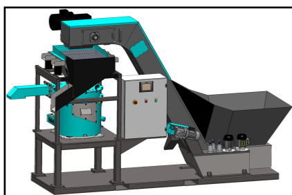
KOMBI-40 D VASCA DRAGATA - DRED. TANK
