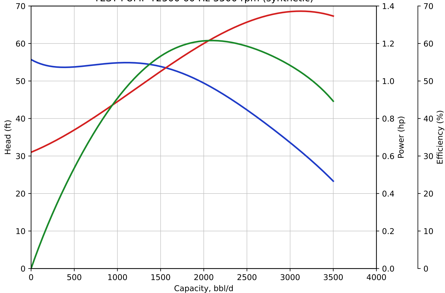
TEST PUMP T2500 60 Hz 3500 rpm (synthetic)
