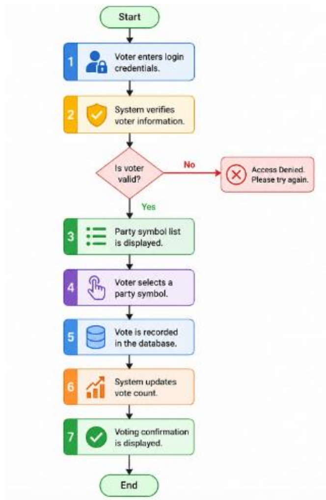
Figure 4. Flowchart
