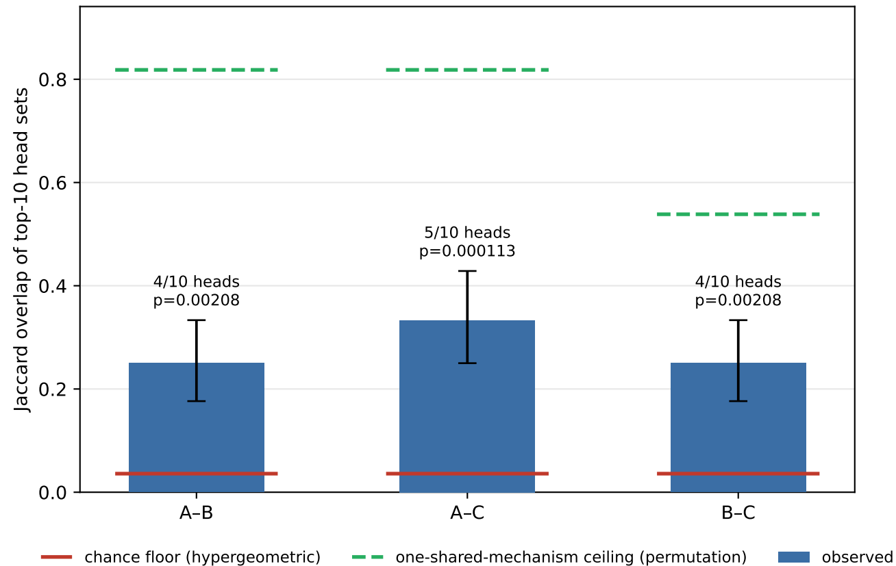
Arbitration head overlap vs both nulls — gpt2
