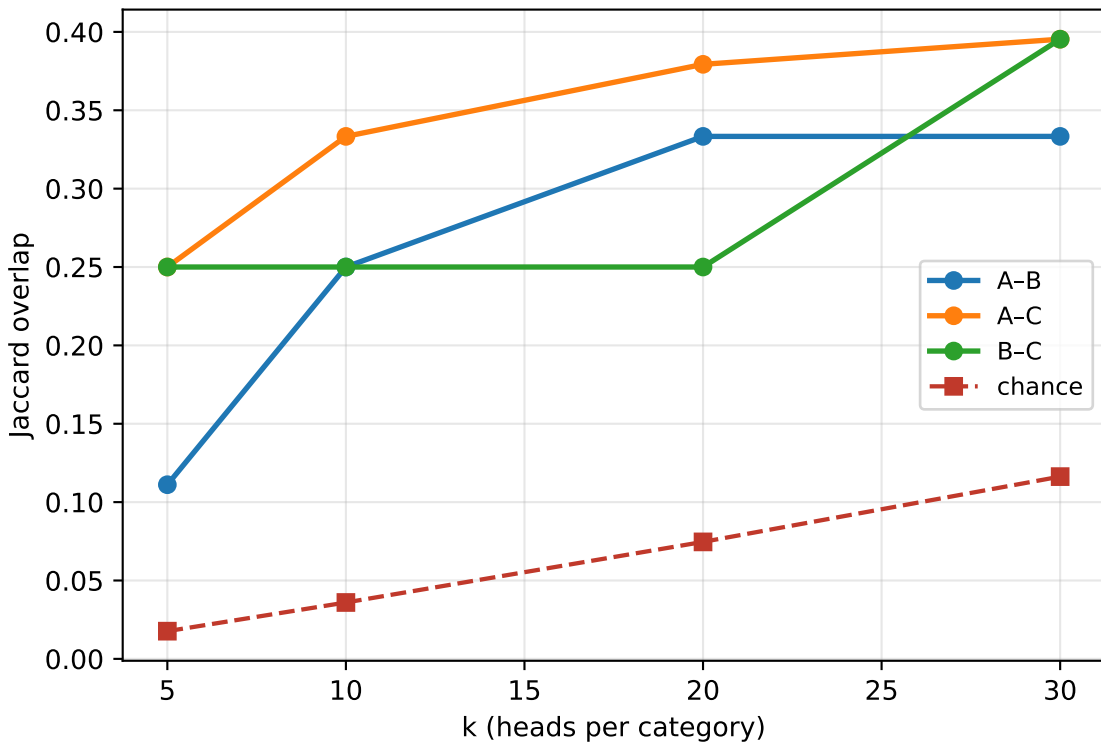
Overlap across selection thresholds — gpt2
