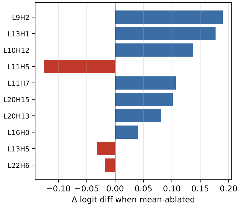
A — coreference
