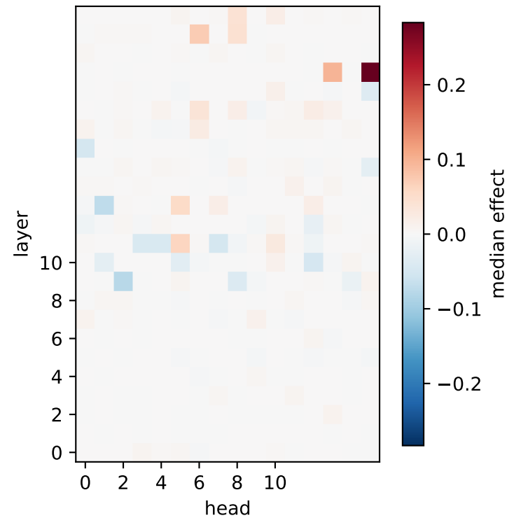
A — coreference
