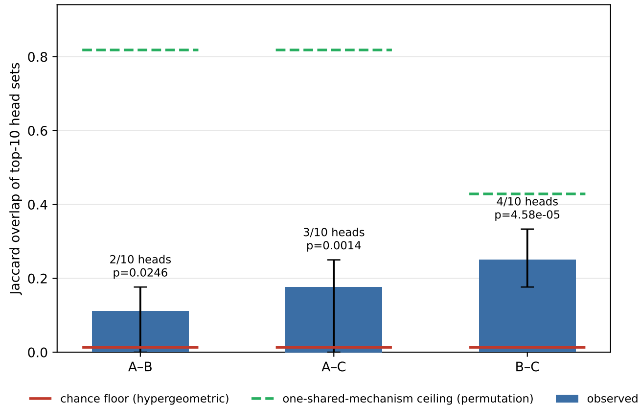
Arbitration head overlap vs both nulls — pythia-410m
