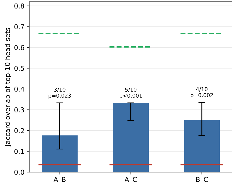
gpt2 (144 heads)
