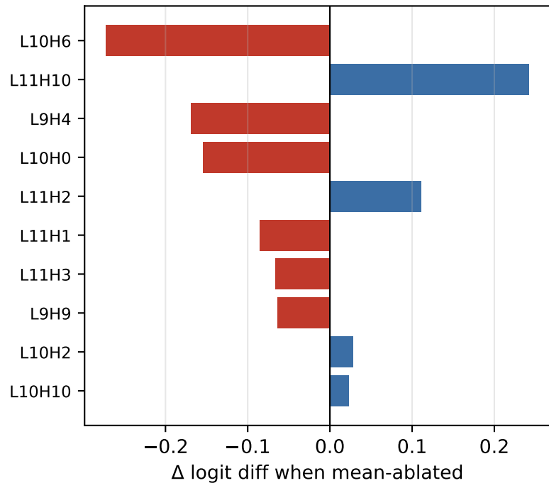
A — coreference
