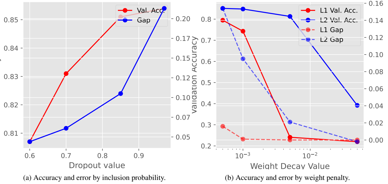
Figure 5. Accuracy and error by regularisation strength of each method (Dropout and L1/L2 Regularisation).
