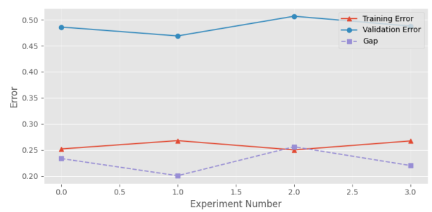
(b) Training and validation error, and generalisation gap for l1+l2 weight penalty.
