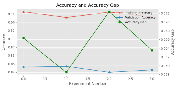
(a) Validation and training accuracy, and generalisation gap for l1+l2 weight penalty.
