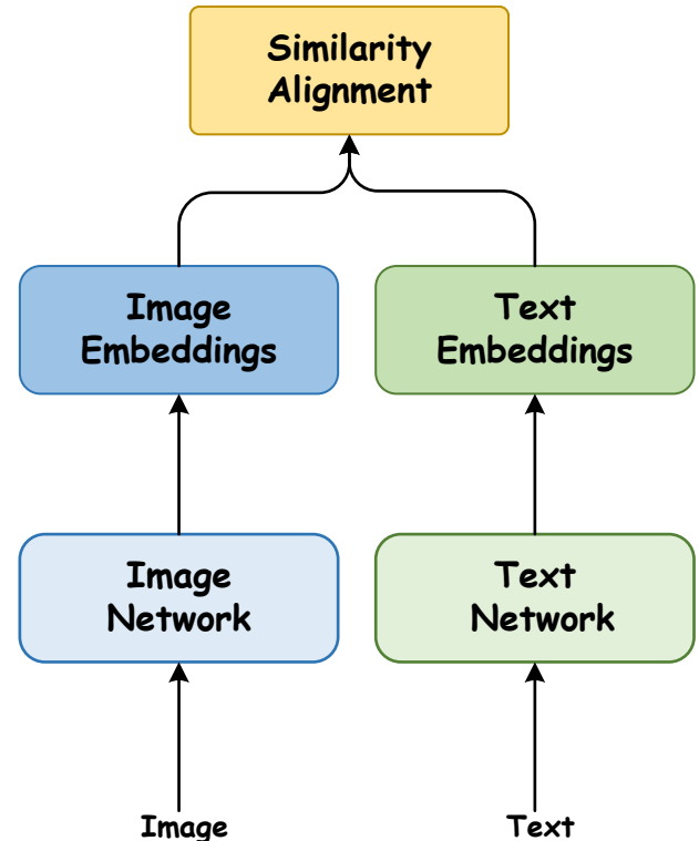
(c) Image-text Alignment
