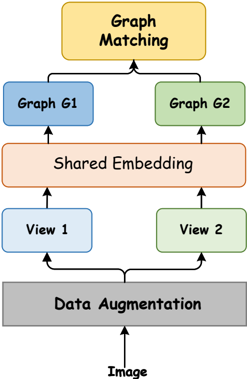
(a) Graph Self-pretraining
