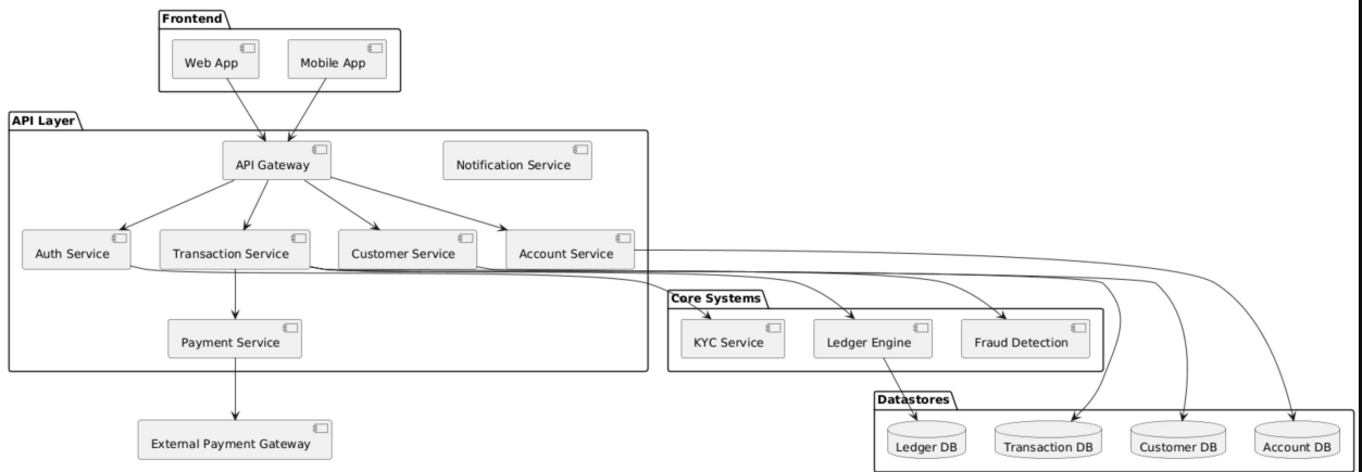
Online Banking - Component Diagram
