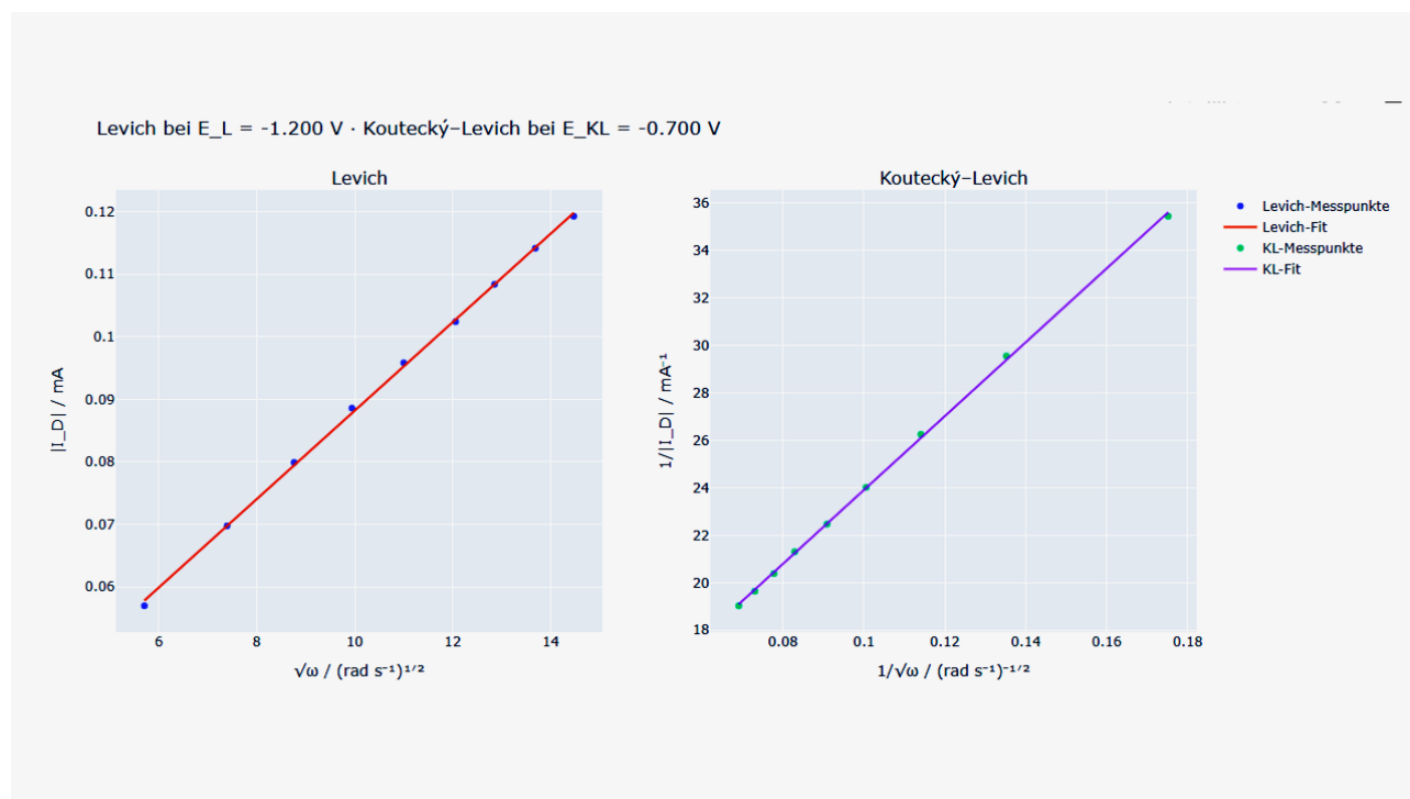
Figure 7: Levich (left) and Koutecky-Levich (right) graphs.
