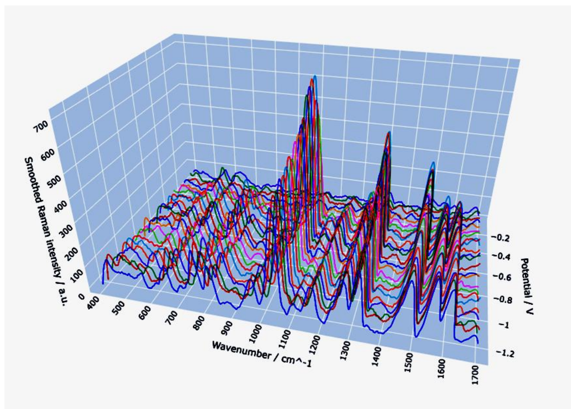
Figure 3: Interactive 3D waterfall plot of Raman spectra of methylene blue recorded at different electrode potentials.
